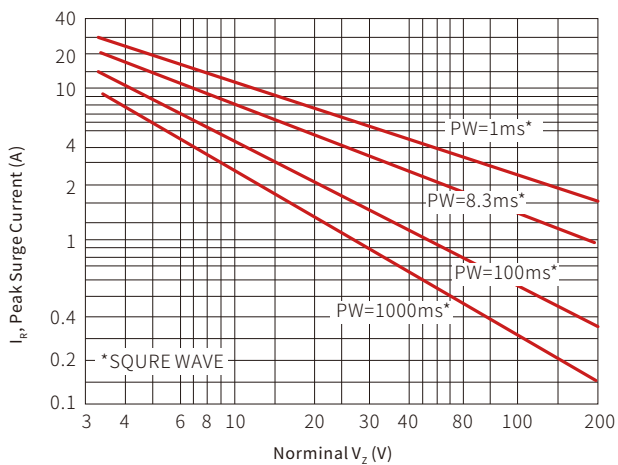
Fig.3-Maximum Non-Repetitive Surg Current Versus Nominal Zener Voltage
