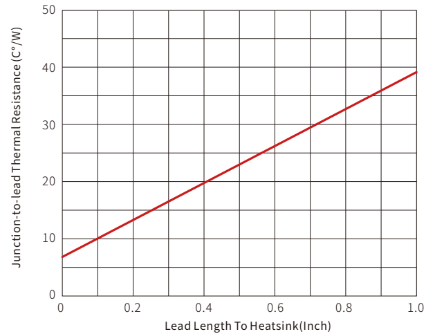
Fig.2-Typical Thermal Resistance
