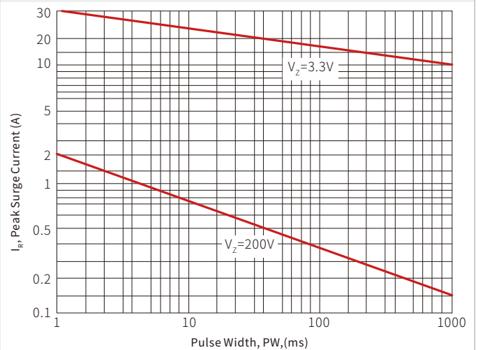
Fig.4-Peak Surg Current Versus Pulse Width
