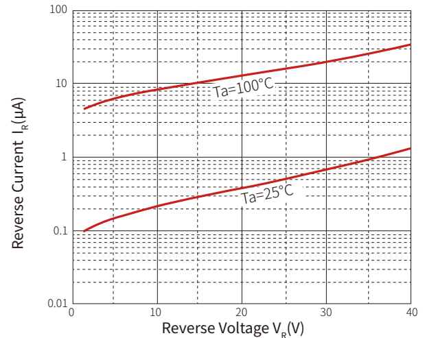
Fig.2 Reverse Characteristics
