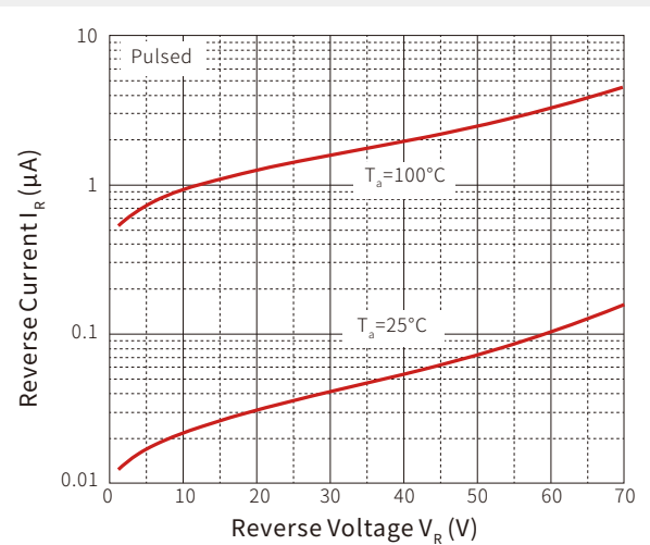
Fig 2. Reverse Characteristics
