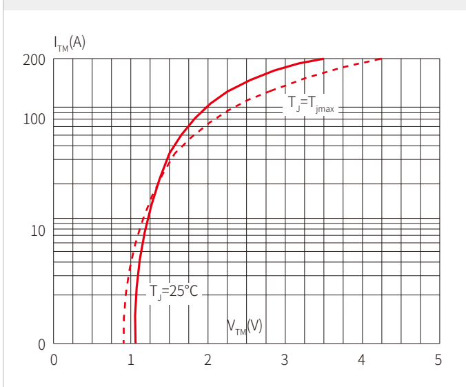
FIG.4 On-state characteristics (maximum values)
