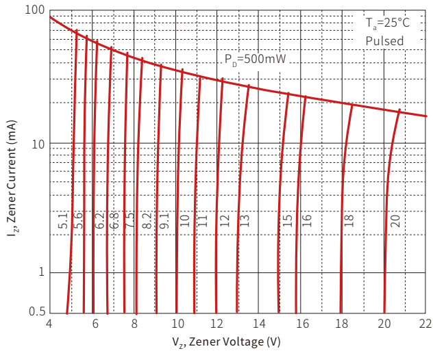
Zener Characteristics ( V_Z Up to 10 V)
