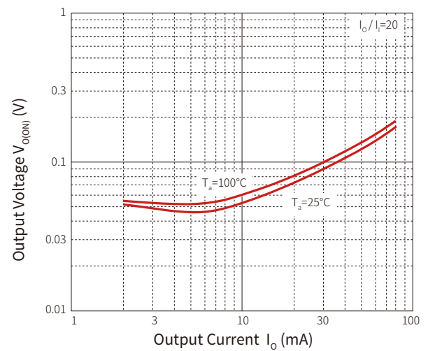
Fig.4 V_{O(ON)} — I_O
