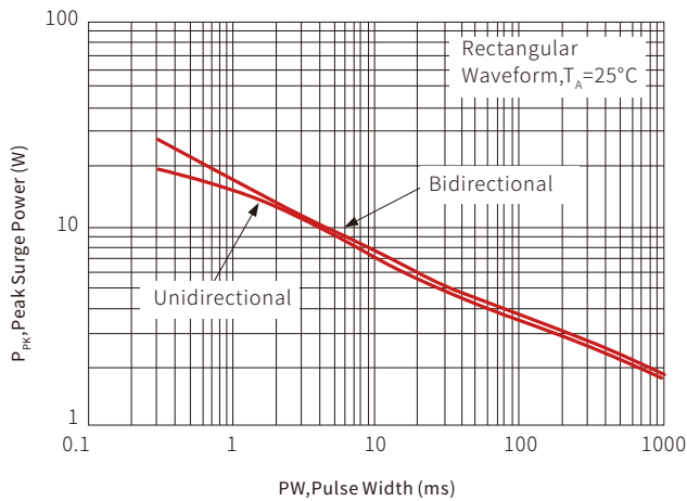
Maximum Non-Repetitive Surge Power, P_{PK}(NOM) Versus PW
