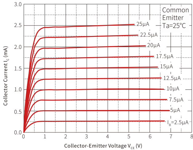
Static Characteristic
