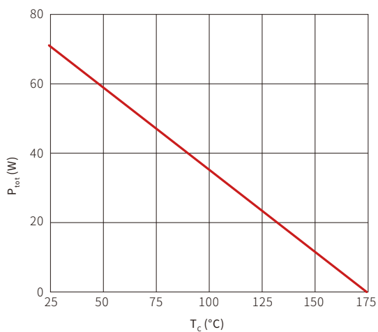
Fig. 7-Power Derating
