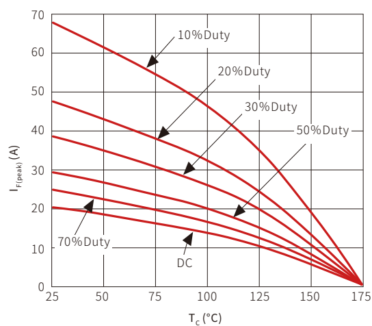
Fig. 8-Current Derating
