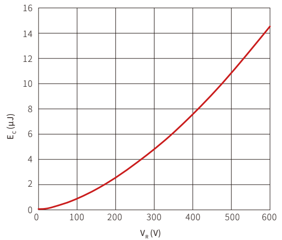
Fig. 6-Capacitance Stored Energy
