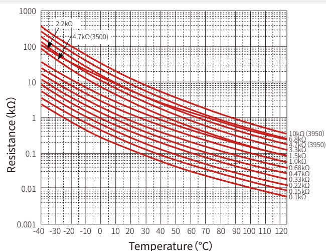
Fig.1 0603 Series (0.1kΩ-10kΩ)
