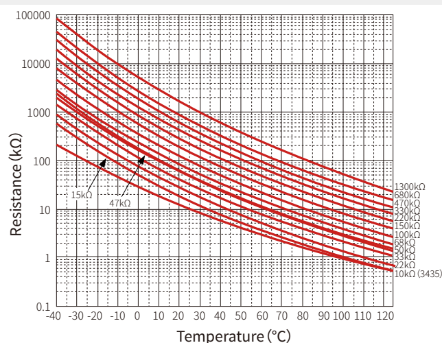
Fig.2 0603 Series (10kΩ-1300kΩ)
