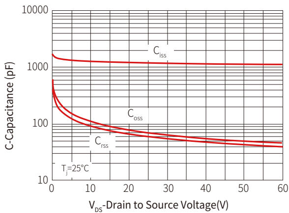
Figure 3: Capacitance Characteristics
