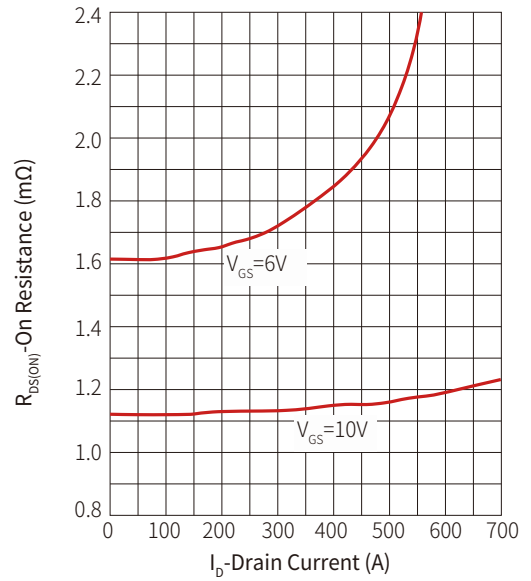
Figure 6: On Resistance
