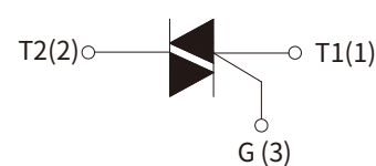
Schematic Symbol
