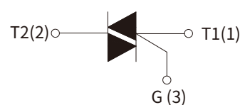
Schematic Symbol
