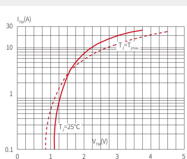
FIG.4 On-state characteristics (maximum values)
