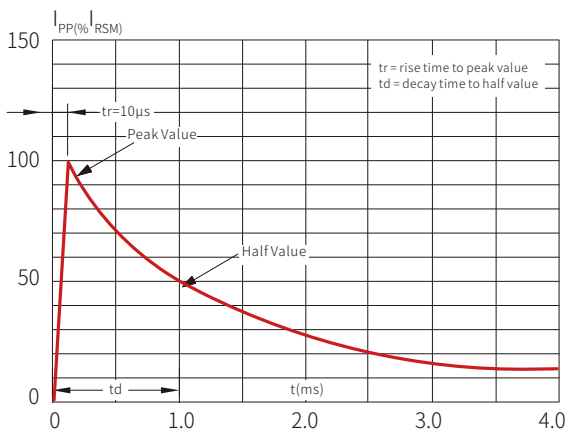
Figure 1: Pulse waveform
