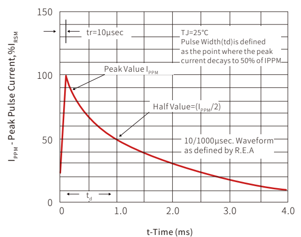
Pulse Waveform
